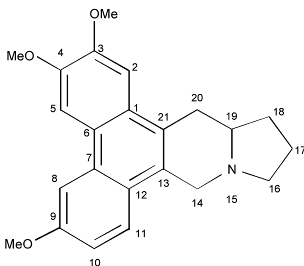
Fig. 1. Chemical structure of (–)-antofine.
