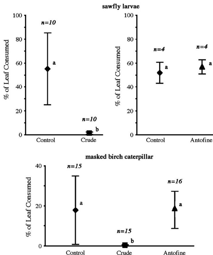
Fig. 2. Consumption of rose leaflets by sawfly larvae (top) and birch leaves by masked birch caterpillar (bottom) after treatment with carrier solvent (control), crude extract of V. rossicum root and (–)-antofine. Each trial consisted of a larva individually enclosed with treated or untreated leaflets/leaves. Means with the same lowercase letter were not significantly different according to a two-tailed t -test (top) or a Tukey–Kramer HSD post-hoc test; \alpha = 0.05 (bottom).
