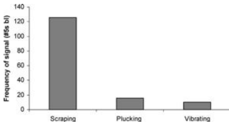
Fig. 8. Frequency of signal use by C. serotiniella larvae. During the staged encounter trials, signaling behavior was observed for a total of 152 5SB. Eighty-three percent of that time was spent scraping, 11% was spent plucking, and 7% was spent vibrating.
